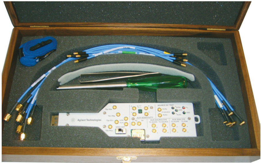
Figure 20. The Agilent W2641B DisplayPort test point adapter fixture
